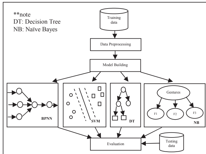
Figure 2. Overview of the proposed system
